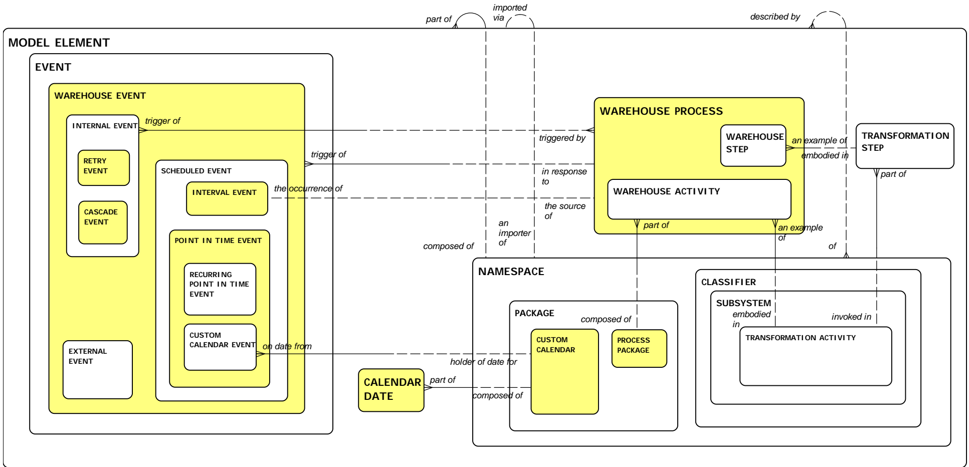
Diagram : FIGURE 4.28 WAREHOUSE PROCESS PACKAGE Modified : 15 September 2002 15:39:52 Author : Copyright © 2002 David C. Hay
